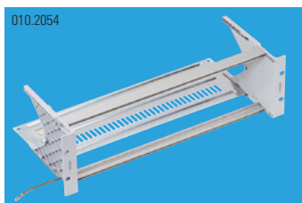
19" 3U Global Patch Panel 60-Port/s, empty
