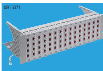
19" 3U Global Patch Panel 60xRJ45/s, Cat.6 A ISO, fully populated
