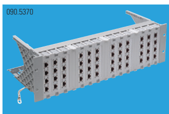
19" 3U Global Patch Panel 48xRJ45/s, Cat.6 A ISO, partly populated
