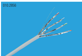
Installation Cable Real10 Cat.6 A , U/FTP, 4P, 650 MHz, LSZH, 500 m
