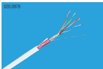
Installation Cable Cat.6 A , F/UTP, 4P, 500 MHz, LSZH, 500 m
