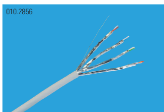
Installation Cable Real10 Cat.6 A , U/FTP, 4P, 650 MHz, LSFRZH, 500 m
