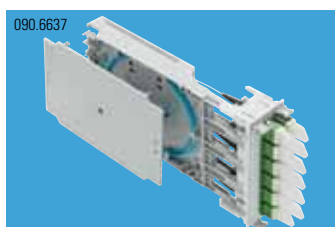
FiberModul HD, breakout, 12xE-2000™ Singlemode, APC, ceramic, black
