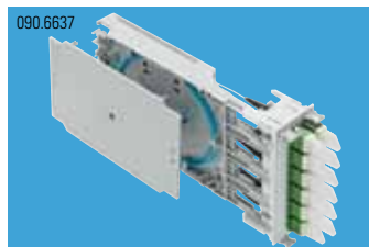
FiberModul HD, breakout, 12xSC Singlemode, APC, ceramic
