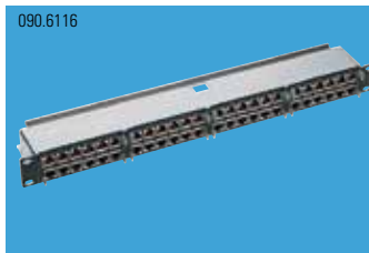
19" 1U HD Basic Patch Panel 48xRJ45/s, Cat.6 A ISO, black, fully populated
