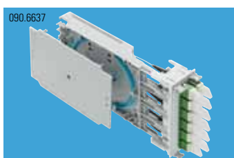
FiberModul HD, breakout, 12xSC Singlemode, APC, ceramic, black
