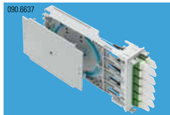
FiberModul HD, breakout, 6xLC-Duplex singlemode, APC, ceramic
