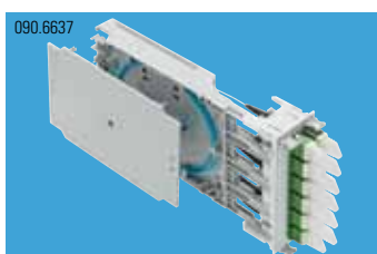
FiberModul HD, breakout, 6xLC-Duplex Singlemode, APC, ceramic, black
