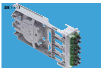
FiberModul HD, breakout, 6xSC-Duplex Singlemode, APC, ceramic
