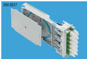
FiberModul HD, breakout, 12xE-2000™ singlemode, APC, ceramic
